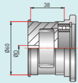
Sealing case 100700-7101-01
