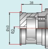
Sealing case 302200-7101-01
